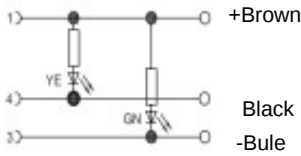
circuit 1
