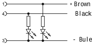
circuit 2
