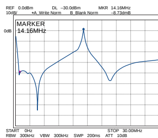
DIGI-SEL Characteristics in 14MHz band
